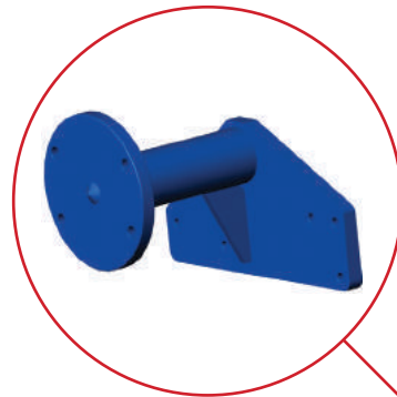
6 Speed Gearbox Bracket Capacity - 350 kg
